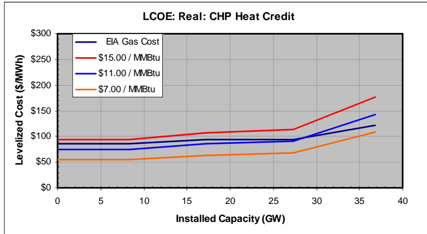
Figure 4: Real Levelized Cost of Energy (LCOE) Including a CHP Heat Credit
