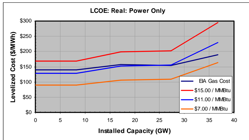
Figure 5: Real Levelized Cost of Energy (LCOE), Power Only (Not Including a CHP Heat Credit)
