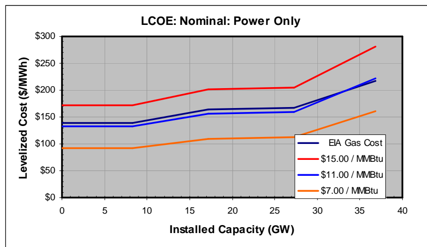
Figure 3: Nominal Levelized Cost of Energy (LCOE), Power Only (Not Including a CHP Heat Credit)
