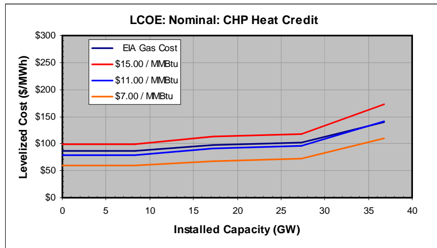
Figure 2: Nominal Levelized Cost of Energy (LCOE) Including a CHP Heat Credit
